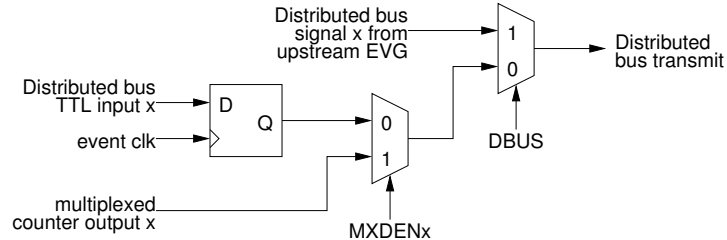
Figure 7: Distributed Bus
